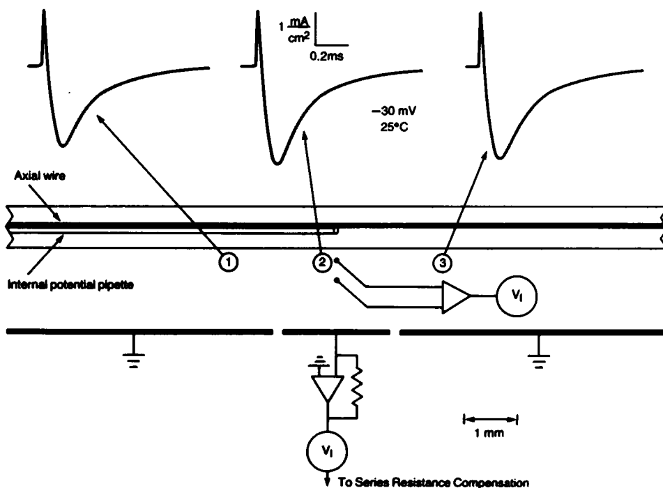
FIGURE 1 Method of current measurement. Not drawn to scale in the vertical direction; a typical axon diameter is 200\ \mu\text{m} , and the external platinum plate ground electrodes were usually \sim 3\ \text{mm} from the axon. The currents shown were recorded at three positions: with the differential electrode opposite the control point (1), 2 mm to the left (2), and 2 mm to the right (3). The nearer wire of the electrode was \sim 700\ \mu\text{m} from the axon. Current density was calculated by comparing current signals recorded with the differential electrode with those from the central plate; in this axon, the calibrating factor was 1\ \text{mA}/\text{cm}^2 for 0.73\ \text{mV} between the wires in the differential electrode. Full Na, Full K, 1\ \text{mM} 4-AP, 2.5^\circ\text{C} .
